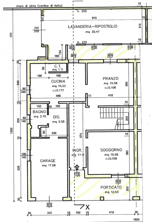
PIANTA PIANO SC
