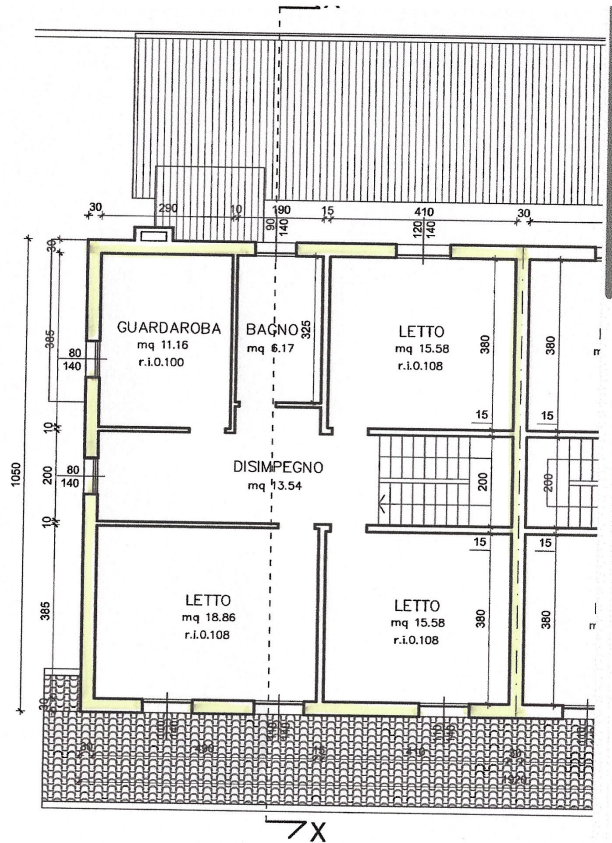
PIANTA PIANO PF
